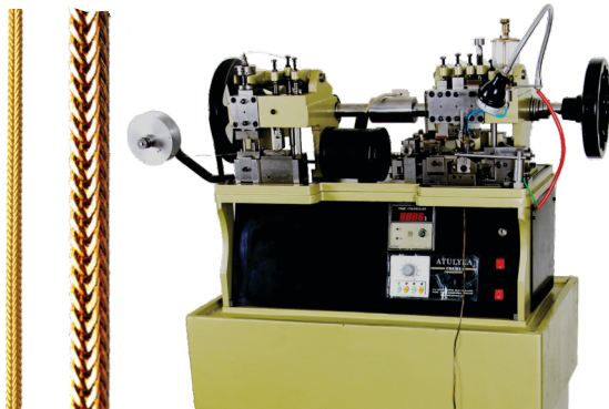
FOX TAIL CHAIN MAKING MACHINE
