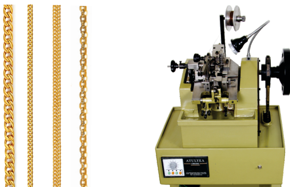
CURB & CABLE CHAIN MAKING MACHINE
